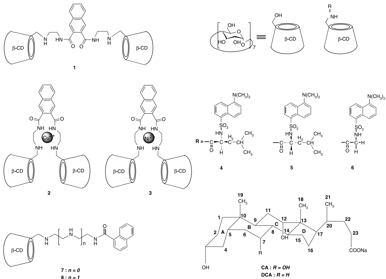
Scheme 1. Molecular structures of host and guest.
