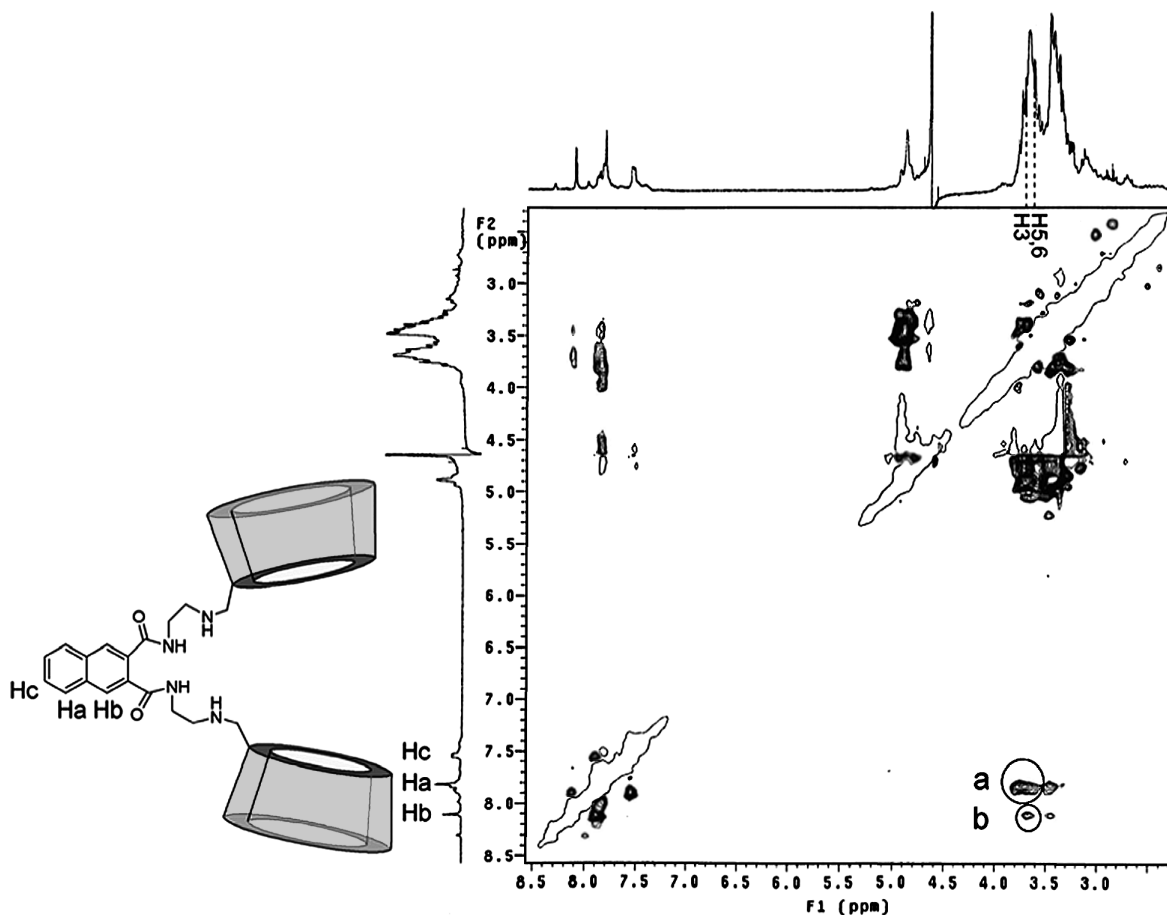
Figure 2. ROESY spectrum of 1 ( 5.0 \times 10^{-3} \text{ mol dm}^{-3} ) in \text{D}_2\text{O} at 25^\circ\text{C} with a mixing time of 300 ms.
