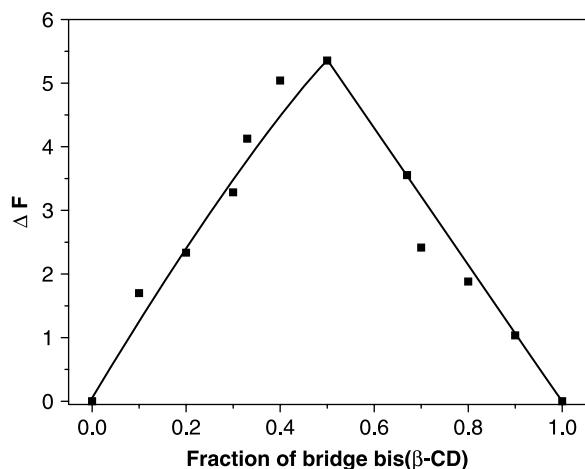
Figure 4. Job's plot of 1 /CA system at 375 nm ( [1] + [CA] = 1.0 \times 10^{-4} \text{ mol dm}^{-3} ).
