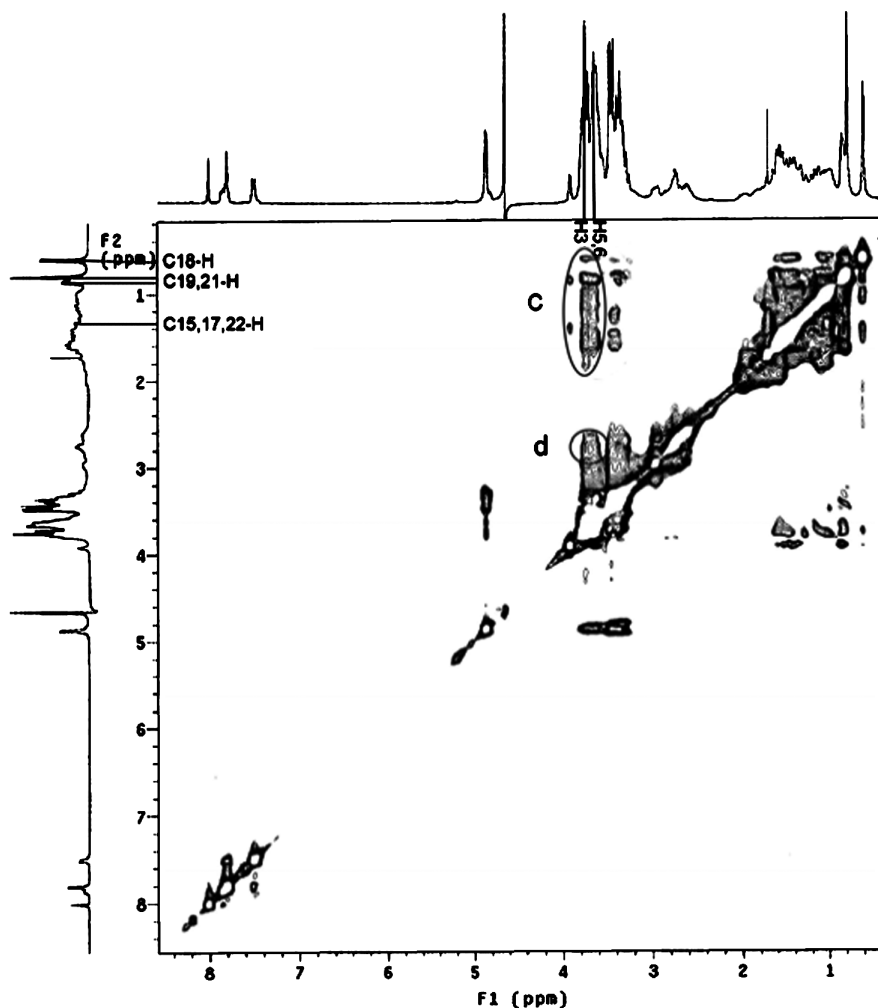
Figure 5. ROESY spectrum of 1 /DCA system ( [1] = [DCA] = 5.0 \times 10^{-3} \text{ mol dm}^{-3} ) in \text{D}_2\text{O} at 25^\circ\text{C} with a mixing time of 300 ms.
