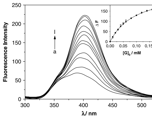
Figure 3. Fluorescence spectral changes of 1 ( 2.0 \times 10^{-6} \text{ mol dm}^{-3} ) with the addition of CA ( 0 , 0.1 \times 10^{-4} , 0.2 \times 10^{-4} , 0.3 \times 10^{-4} , 0.4 \times 10^{-4} , 0.5 \times 10^{-4} , 0.6 \times 10^{-4} , 0.8 \times 10^{-4} , 1.0 \times 10^{-4} , 1.2 \times 10^{-4} , 1.4 \times 10^{-4} and 1.6 \times 10^{-4} \text{ mol dm}^{-3} ) in Tris-HCl buffer solution (pH 7.4) and the nonlinear least-squares analysis (inset) to calculate the complex stability constant ( K_s ). The excitation wavelength is 268 nm.
