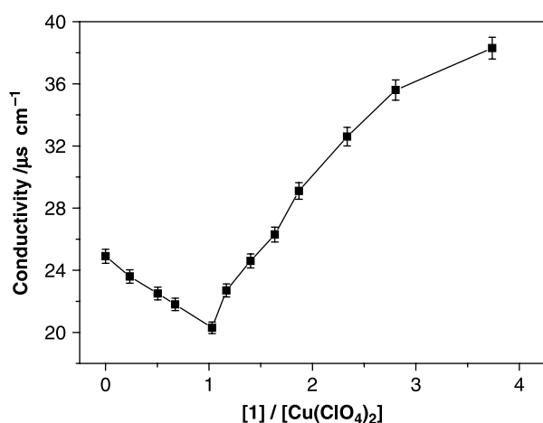
Figure 1. The dependence of conductivity of \text{Cu}(\text{ClO}_4)_2 ( 1.07 \times 10^{-4} \text{ mol dm}^{-3} ) on the concentration of 1 ( 0, 0.25 \times 10^{-4}, 0.54 \times 10^{-4}, 0.72 \times 10^{-4}, 1.1 \times 10^{-4}, 1.25 \times 10^{-4}, 1.5 \times 10^{-4}, 1.75 \times 10^{-4}, 2.0 \times 10^{-4}, 2.5 \times 10^{-4}, 3.0 \times 10^{-4} and 4.0 \times 10^{-4} \text{ mol dm}^{-3} ) in aqueous solution at 25^\circ\text{C} .
